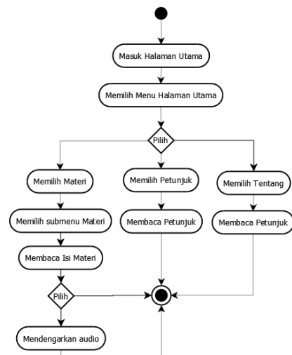
Gambar 2. Activity Diagram Aplikasi Kitab Arba'in Nawawi Berbasis Android
